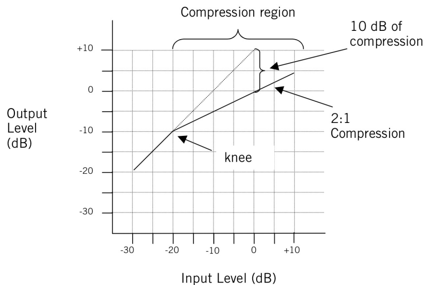
INPUT/OUTPUT CURVE OF A COMPRESSOR WITH A RATIO OF 2:1 AND A THRESHOLD OF -20 DB.
