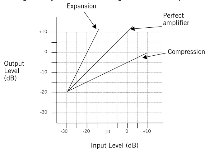
INPUT/OUTPUT CHARACTERISTICS OF A COMPRESSOR, AN EXPANDER AND A PERFECT AMPLIFIER.
