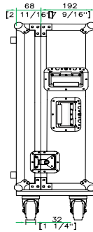
RIGHT VIEW
