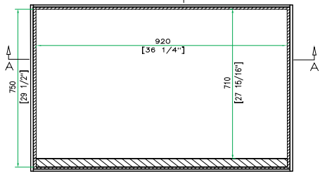
TOP VIEW OF COVER
