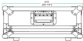
BACK VIEW
