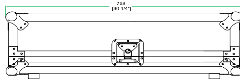
RIGHT VIEW
