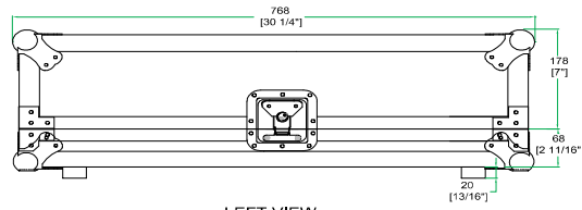
LEFT VIEW
