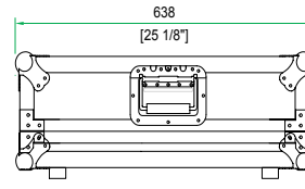
RIGHT VIEW
