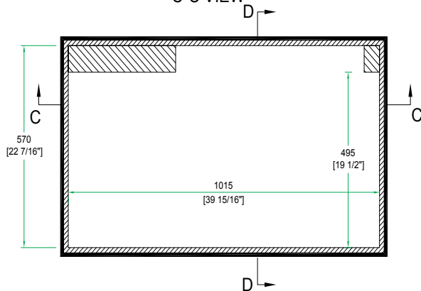
TOP VIEW OF BASE
