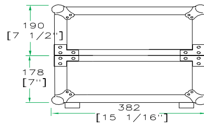
LEFT VIEW
