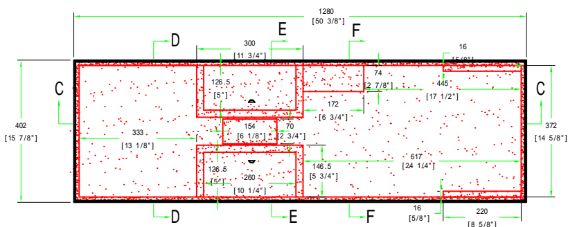
TOP VIEW OF BASE
