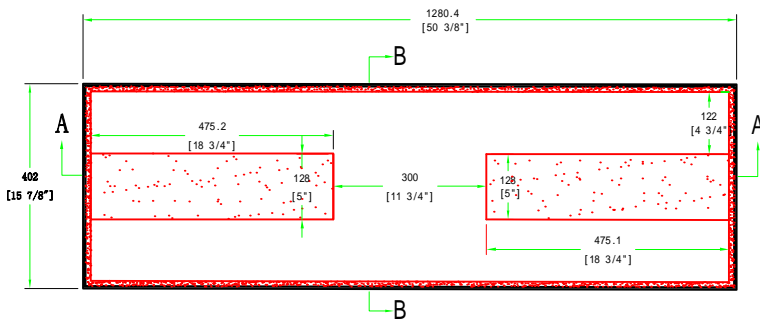
TOP VIEW OF COVER
