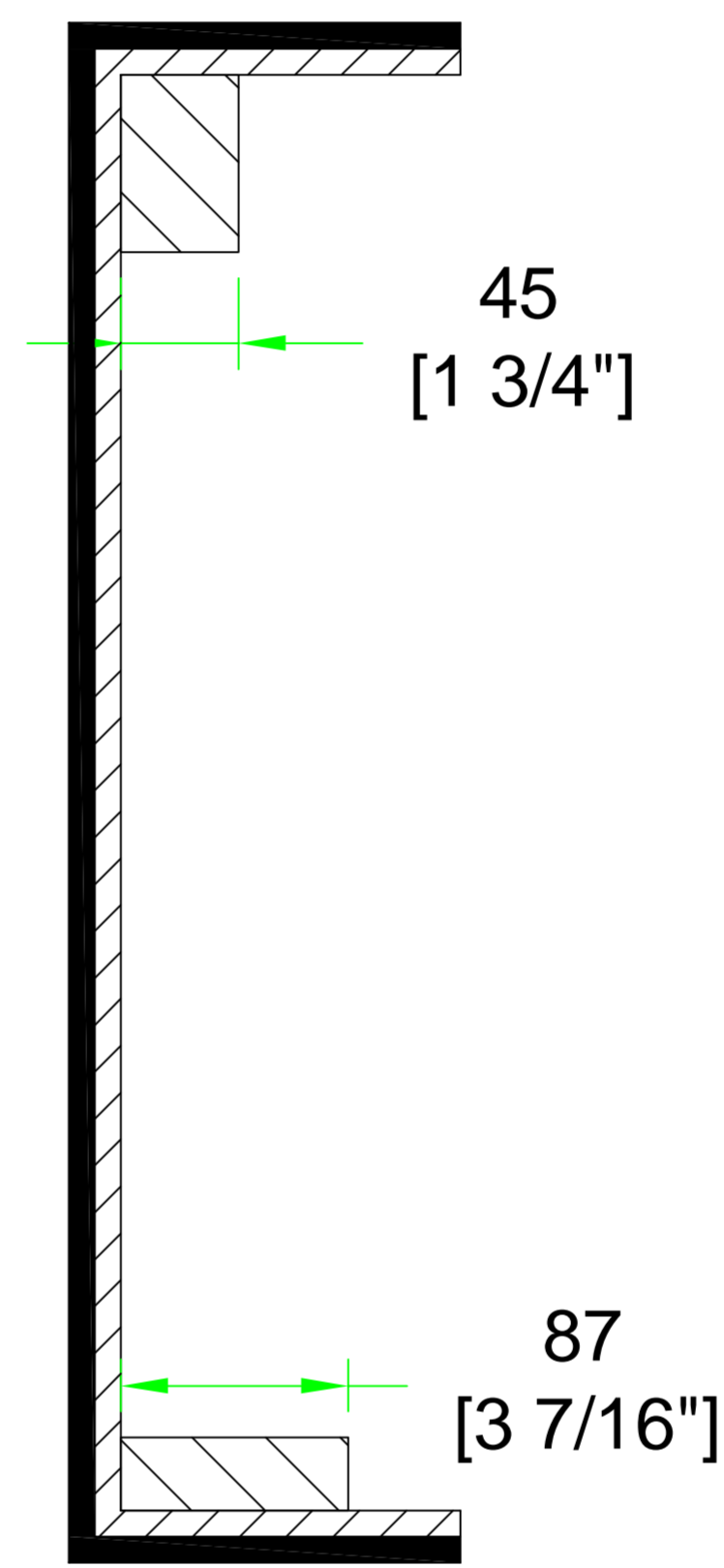
B-B VIEW
