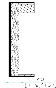
E-E VIEW
