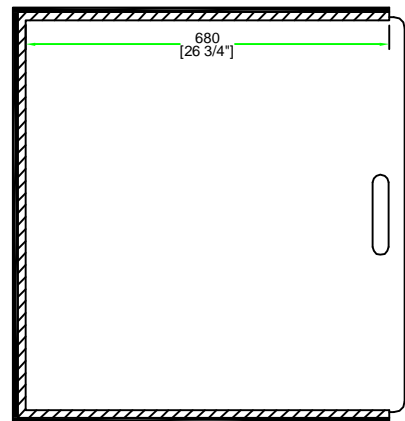
D-D VIEW
