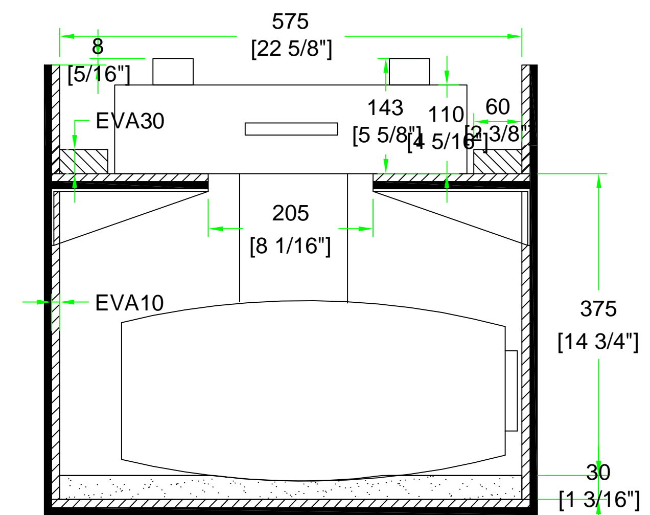
D-D VIEW
