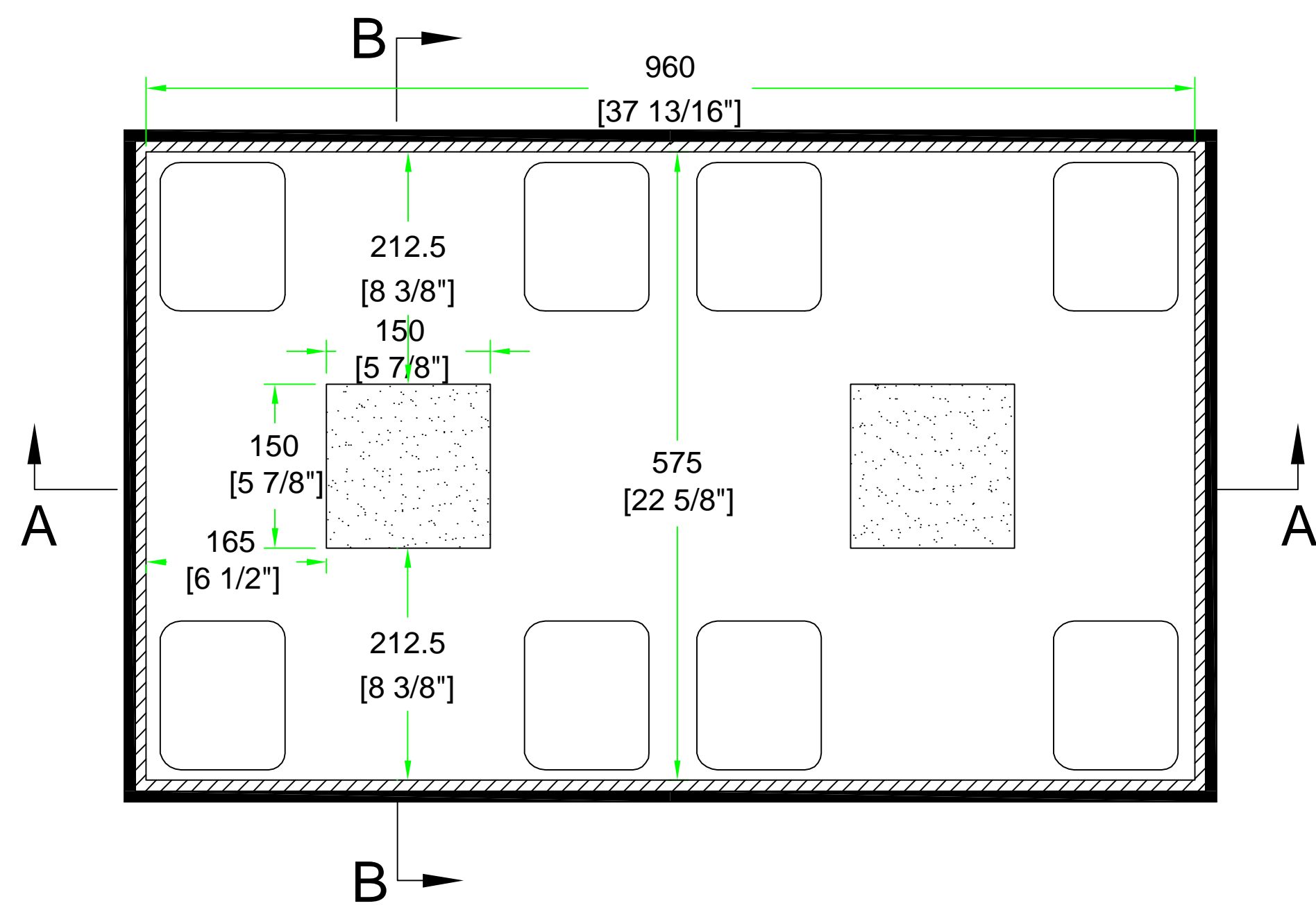
TOP VIEW OF COVER
