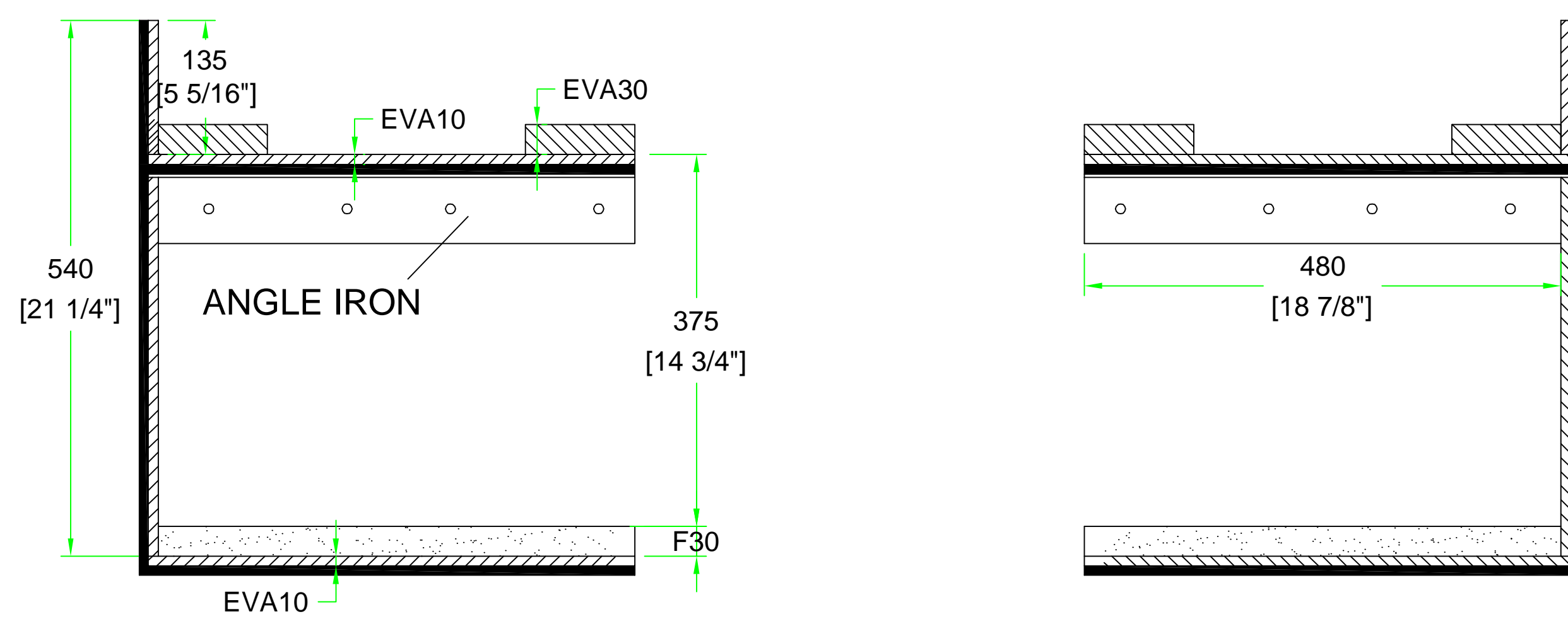
C-C VIEW
