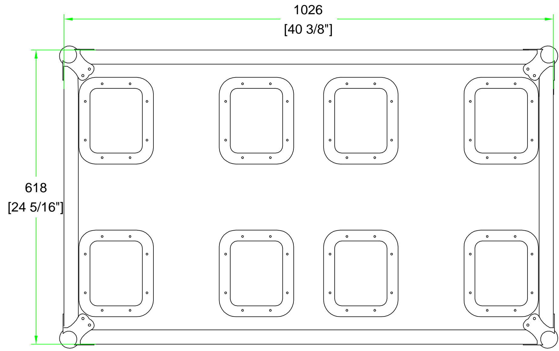
TOP VIEW
