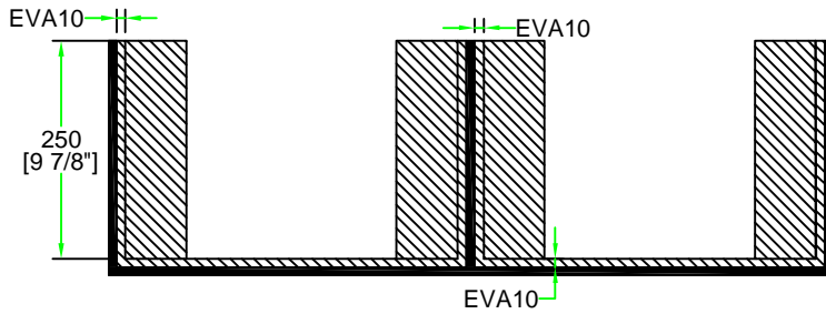
C-C VIEW
