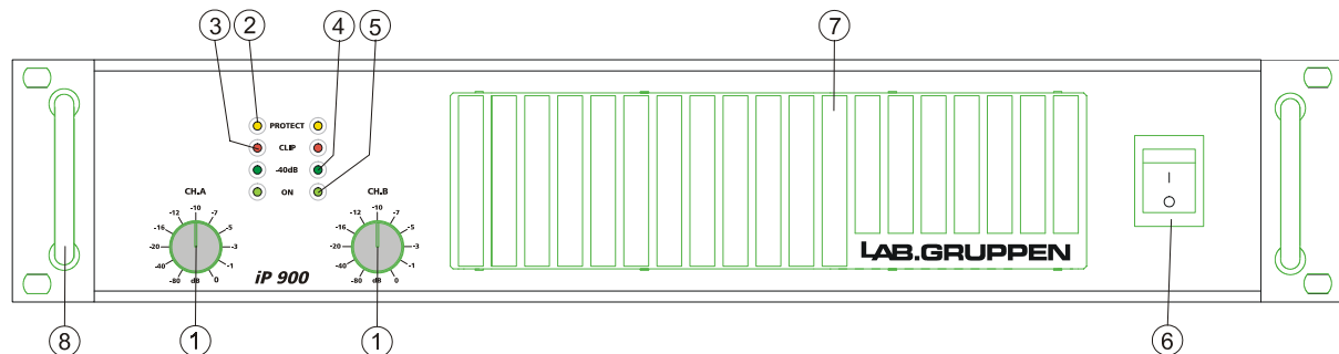
Figure 1 front panel
