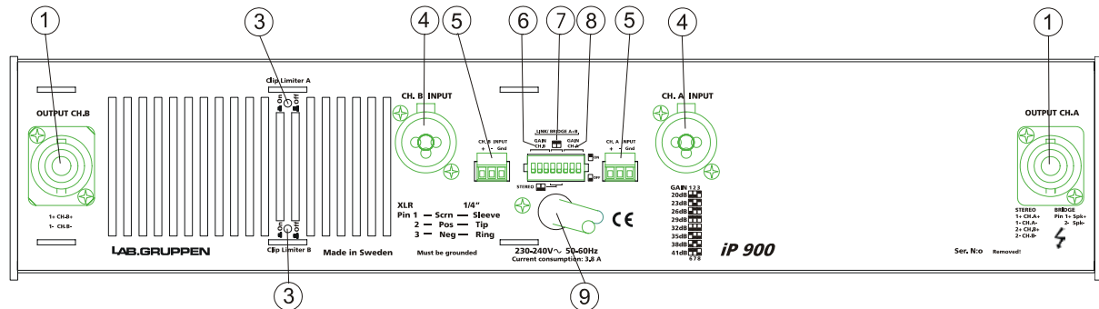
Figure 2. Rear Panel
