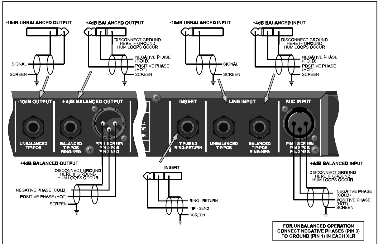
AUDIO CONNECTION DIAGRAM
