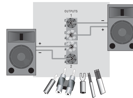
Figure 2.8 Binding Post Output Wiring
