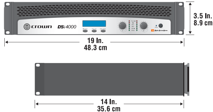
Figure 2.1 Dimensions
