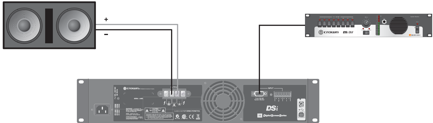
Figure 2.10 Bridge-Mono Wiring
