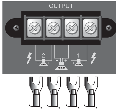
Figure 2.6 Barrier Strip Output Wiring
