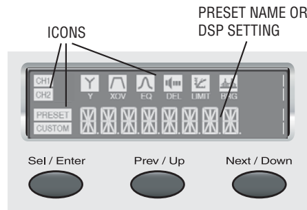
Figure 4.3 LCD Screen and Menu Navigation Buttons
