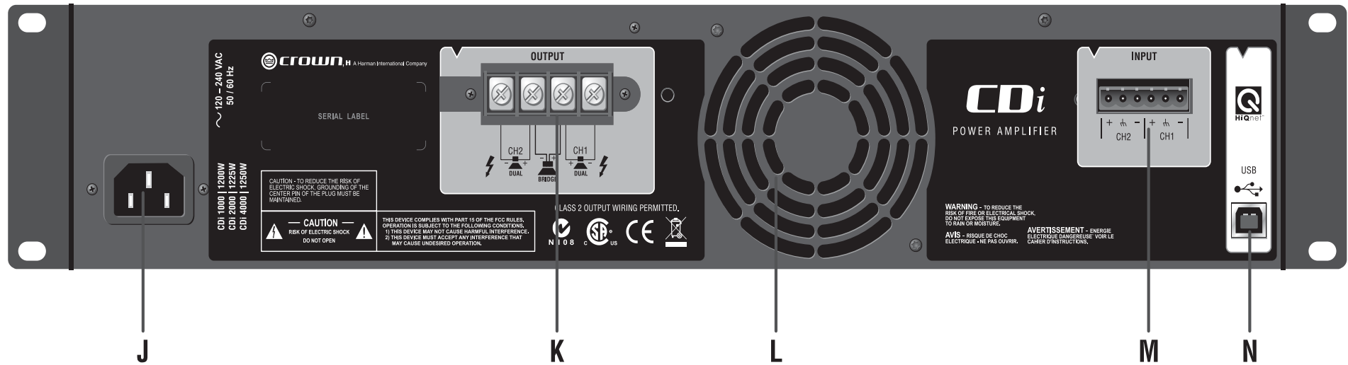
Figure 3.3 Back Panel Connectors
