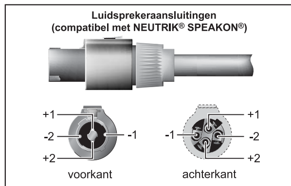
Afb. 1.2: Speakon®-stekker
