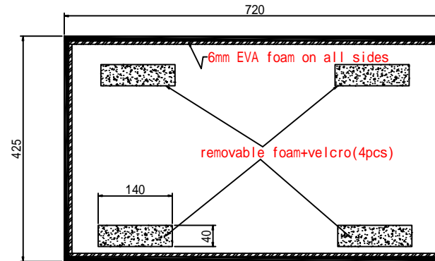
TOP VIEW OF BASE
