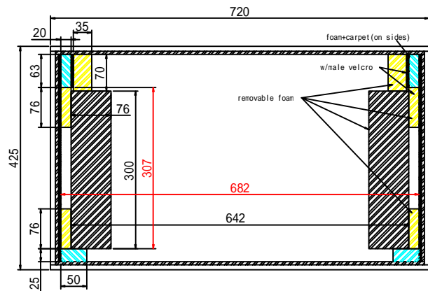
TOP VIEW OF COVER
